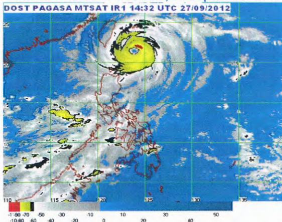
Satellite Picture at 4:32 a.m., 28 September 2012 DOST PAGASA MTSAT IR 1 14:32 UTC 27/09/2012
