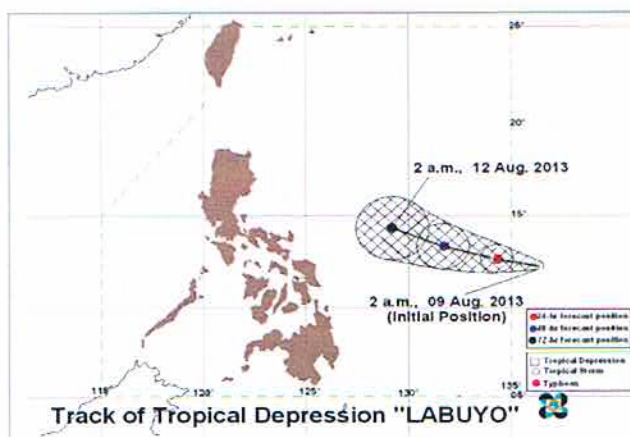
PAGASA Track as of 2 a.m., 09 August 2013
