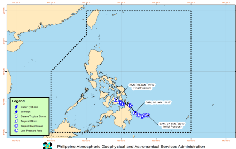
Track of Tropical Depression "AURING"
