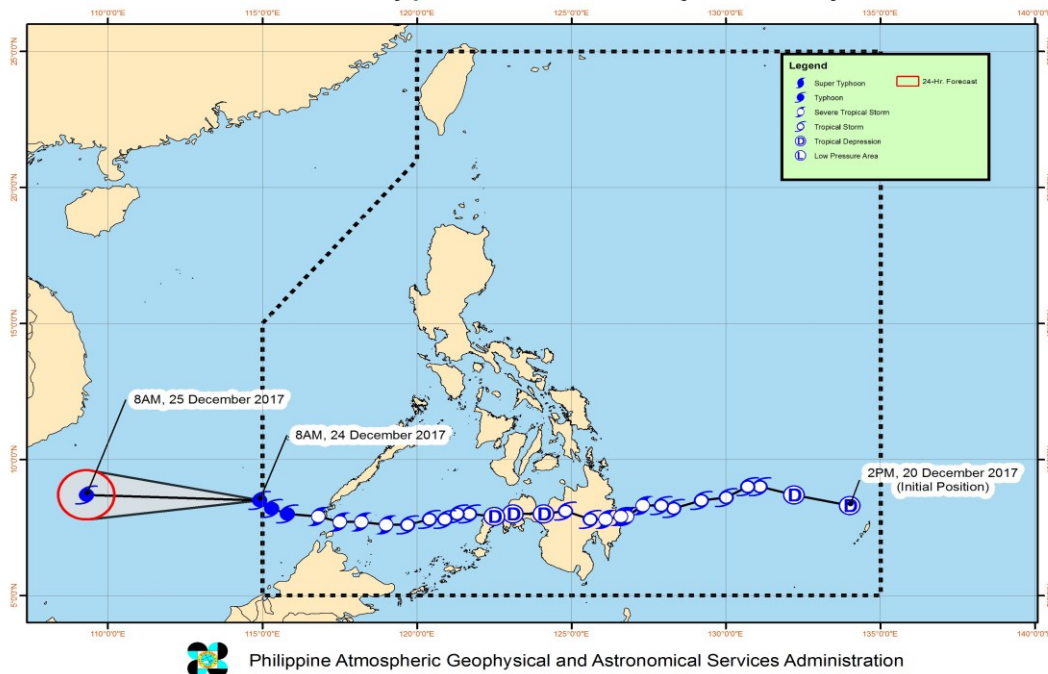
Track of Typhoon "VINTA" {TEMBIN}
